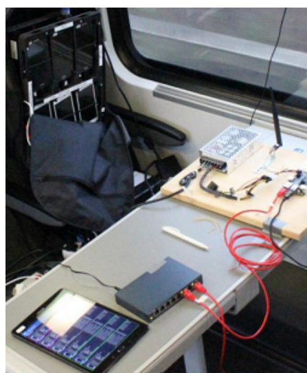
Figure 1: The measurement setup.
